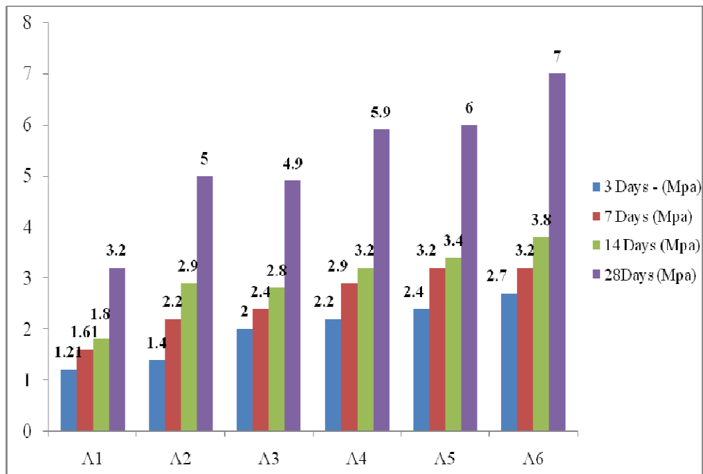
Figure 7 – Compression test comparison
