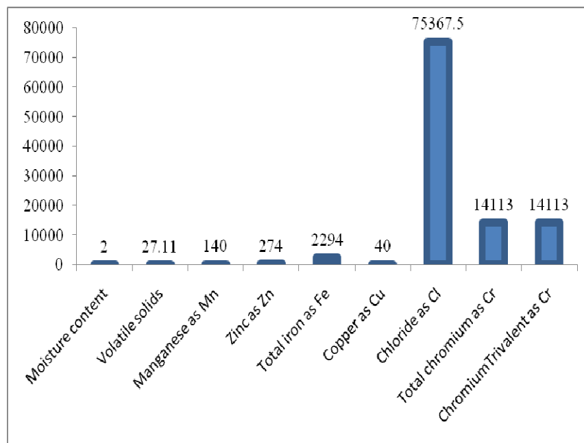
Figure 2 – Physical and chemical characteristics of raw tannery sludge + 10 % lime
