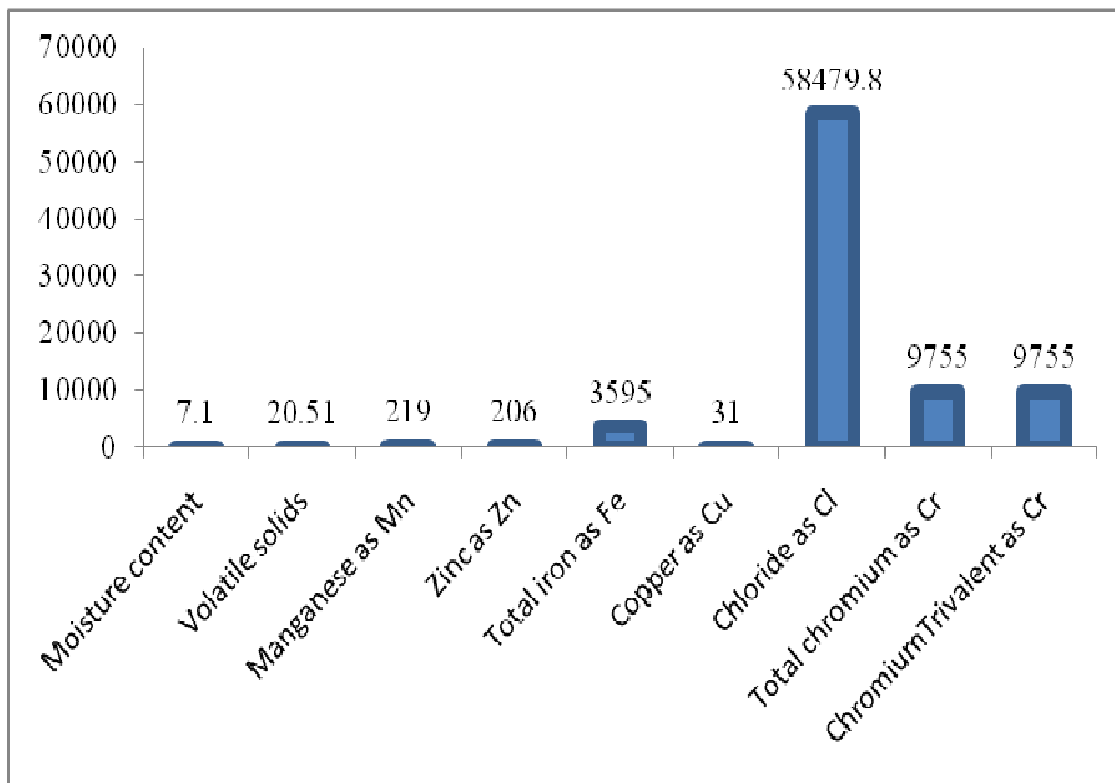
Figure 4 – Physical and chemical characteristics of raw tannery sludge + 30 % lime
