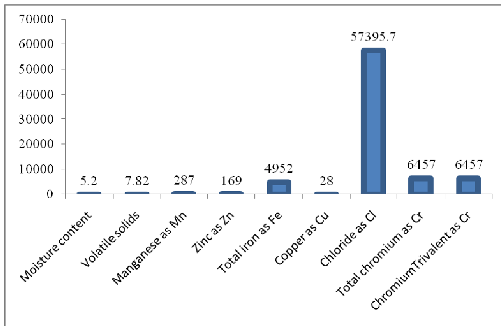
Figure 6 – Physical and chemical characteristics of raw tannery sludge + 50 % lime
